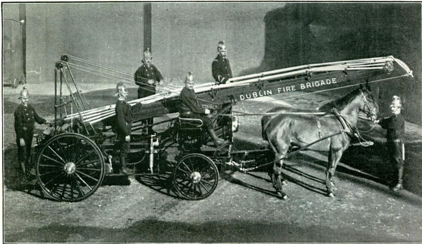
"AERIAL" TURNTABLE EXTENSION LADDER
